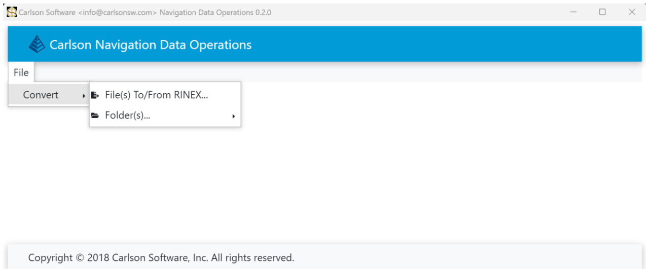
Figure 64 - Nj-ops GUI.
